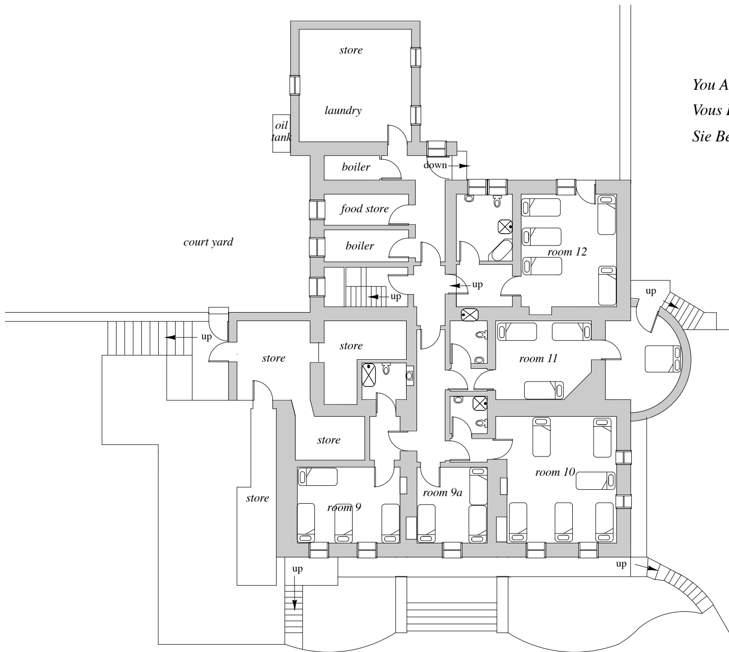
LOWER GROUND FLOOR LAYOUT (not to scale)
